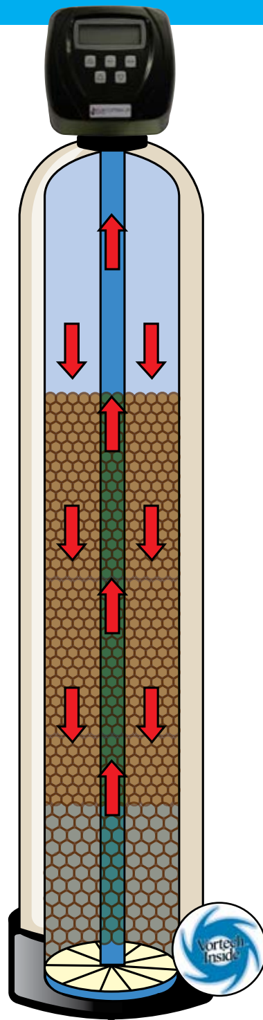
Vortech™ Distributor - Enhanced filter cleaning. Not available in all sizes.
